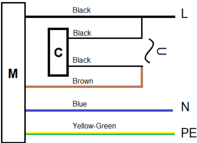
SINGLE-PHASE - WIRING DIAGRAM SKU: 200072 - CCW
